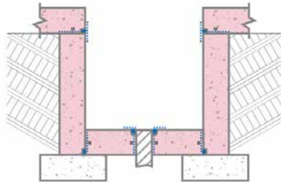
Detail for hydraulic elevator pit construction
