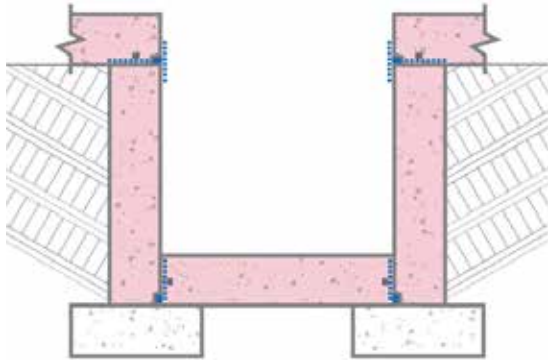
Admix included in the concrete mix
