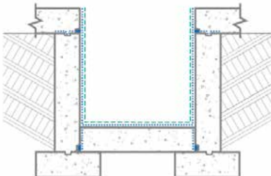
Application of crystalline waterproofing coating on negative side
