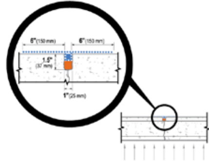
Details for crack or joint sealing (against a flow of water)
