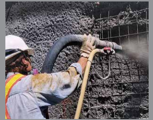
Shotcrete
